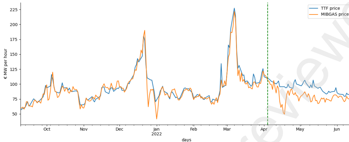
Figure 4: Evolution of gas price: MIBGAS y TTF
